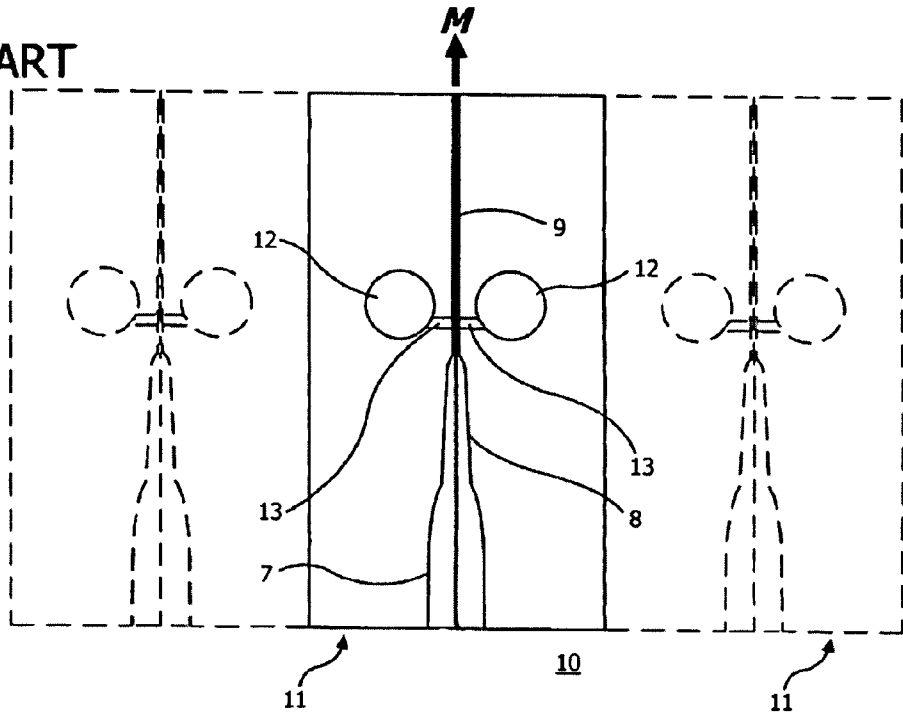
Fig. 6 PRIOR ART
